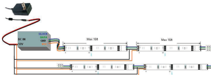
Connection Schematic
