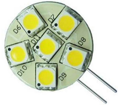
Side pin mounting Wafer
